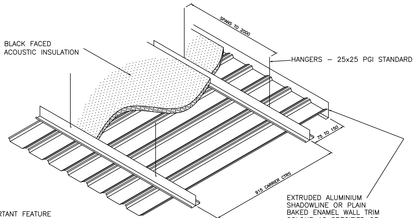
SYSTEM ASSEMBLY
