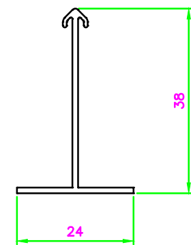
CROSS TEE 600mm
