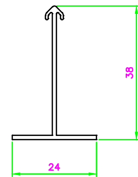
MAIN BEAM
