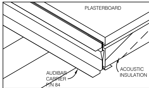
DETAIL "B"
